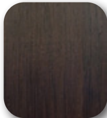
Java
